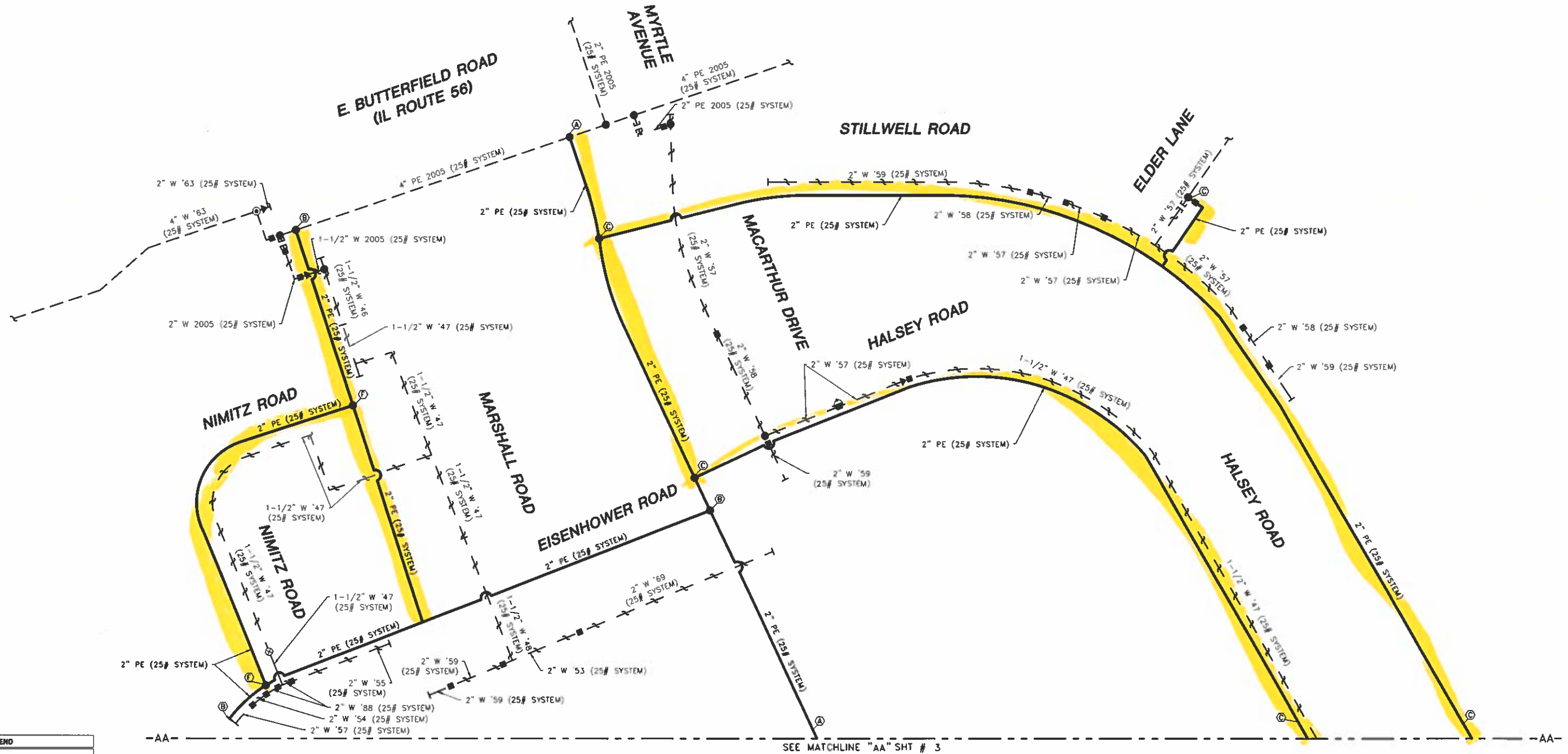
SITE PLAN (1 OF 2) (NOT TO SCALE)
